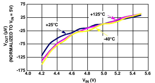
FIGURE 22. LINE REGULATION OVER-TEMPERATURE
