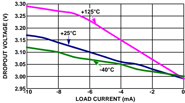
FIGURE 7. LOAD CURRENT vs DROPOUT
