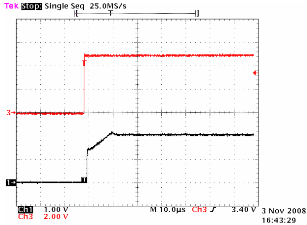
FIGURE 57. TURN-ON TIME, 1kΩ
