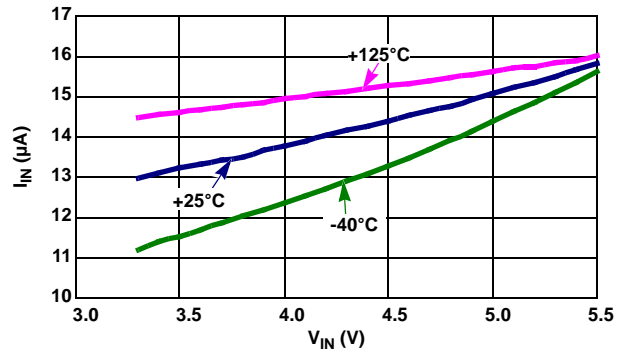
FIGURE 2. I_{IN} vs V_{IN} , 3 TEMPERATURES
