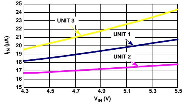
FIGURE 18. I_{IN} vs V_{IN} , 3 TEMPERATURES
